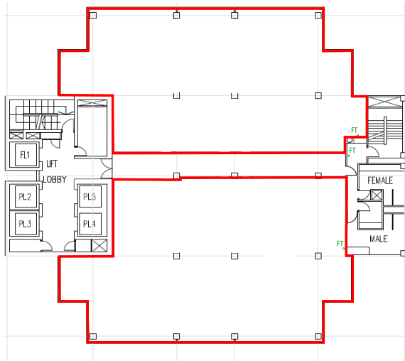
10TH, 11TH, 13TH, 14TH AND 16TH STOREY PLAN WISMA ATRIA
