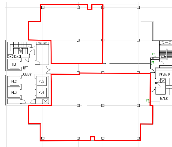
19TH AND 20TH STOREY PLAN WISMA ATRIA
