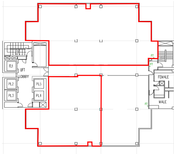
21ST AND 22ND STOREY PLAN WISMA ATRIA
