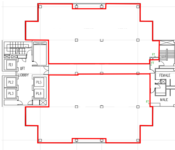
17TH AND 18TH STOREY PLAN WISMA ATRIA
