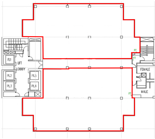
10TH, 11TH, 14TH AND 16TH STOREY PLAN WISMA ATRIA
