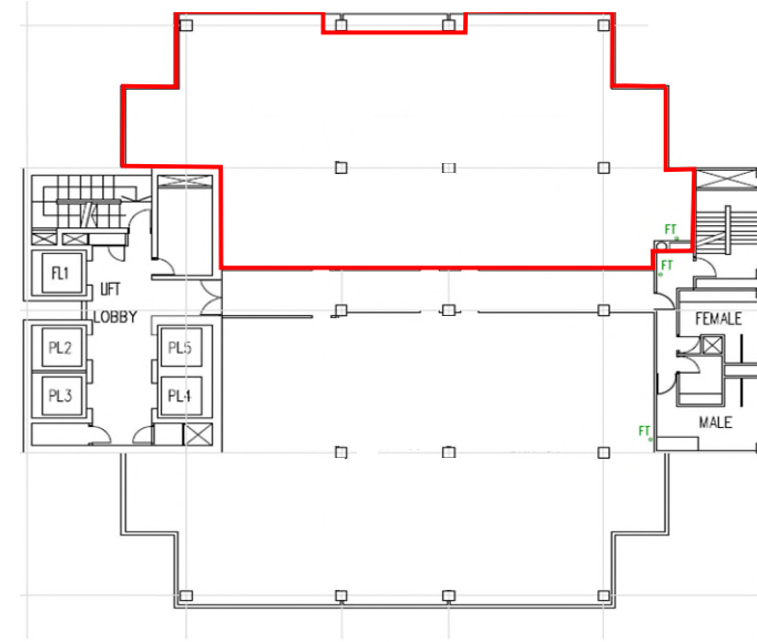
17TH STOREY PLAN WISMA ATRIA
